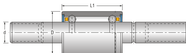
Special double-row bearings type „K“
