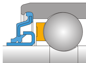
TRIPLE LIP SEAL
