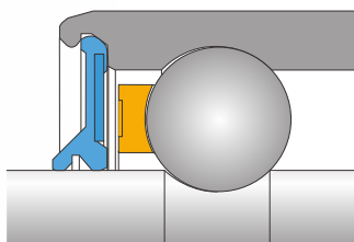
DOUBLE LIP SEAL
