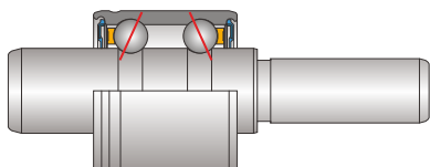
SPECIAL ASYMMETRICAL BEARINGS
